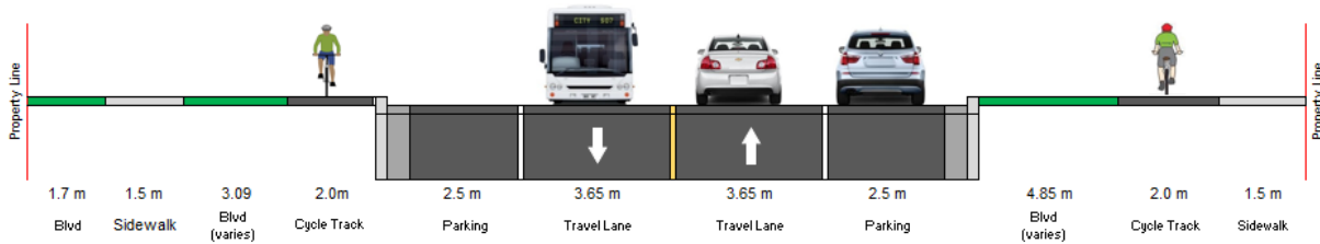
Alternative 3: Cycle Tracks (Representative Cross-Section)
