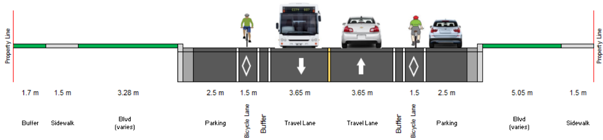
Alternative 2: Buffered Bicycle Lanes (Representative Cross-Section)
