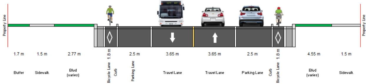
Alternative 1: Physically Protected Bicycle Lanes (Representative Cross-Section)
